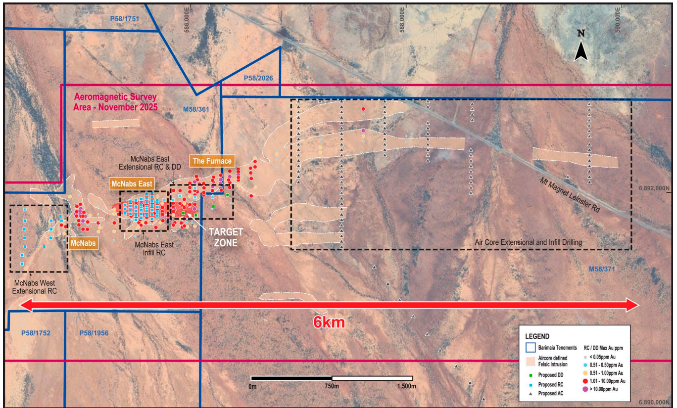
Figure 4. Plan view showing proposed exploration for November to December 2025.
