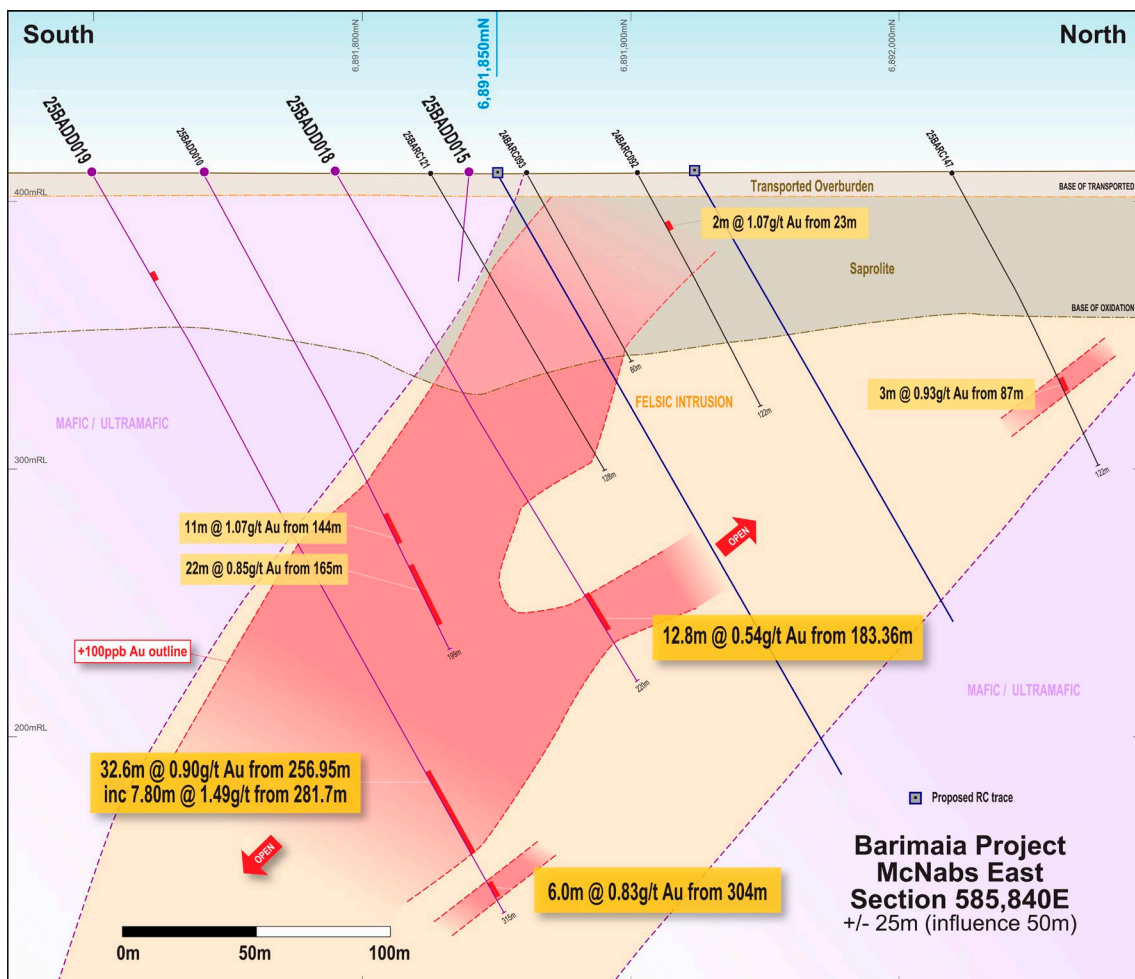
Figure 3. Section 585,840E showing recent diamond drilling intercepts reported in this release. The location of the section line is shown on Figure 1 and Figure 2.
