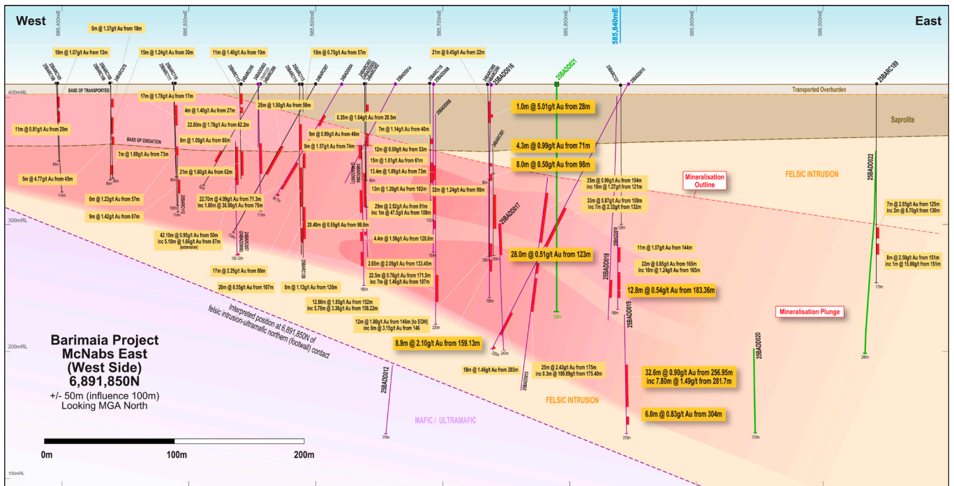
Figure 2. Section 6,891,850N looking north, highlighting an extensive zone of gold mineralisation plunging to the east. The position of the felsic and ultramafic contact at 6,891,850N is shown. This section location is shown on Figure 1 and the position of Figure 3 cross-section 585,840E is shown.
