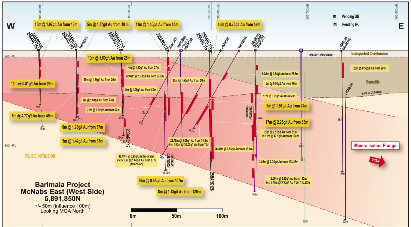
Figure 2. Section 6,891,850N looking north, highlighting a shallow zone of gold mineralisation plunging to the east. March 2025 RC drill intercepts are highlighted in dark yellow boxes. The section location is shown on Figure 1.
