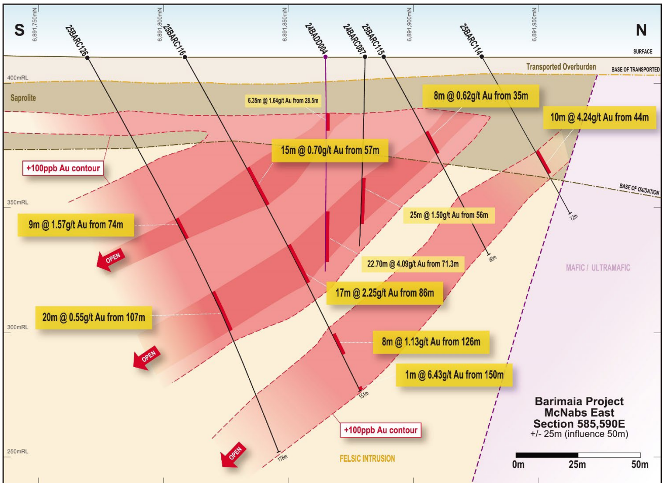
Figure 3. Section 585,590E looking west highlighting high-grade gold mineralisation hosted within the felsic intrusion. The section location is shown on Figure 1.
